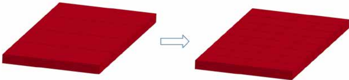
Figure 1. Mesh Fission for Sandwich Structure Part: 32 hexahedral elements are refined to 128 of the same type, as a sweeping of the top and bottom adaptive shell elements through the thickness. The number of layers of the solids always remains the same.
